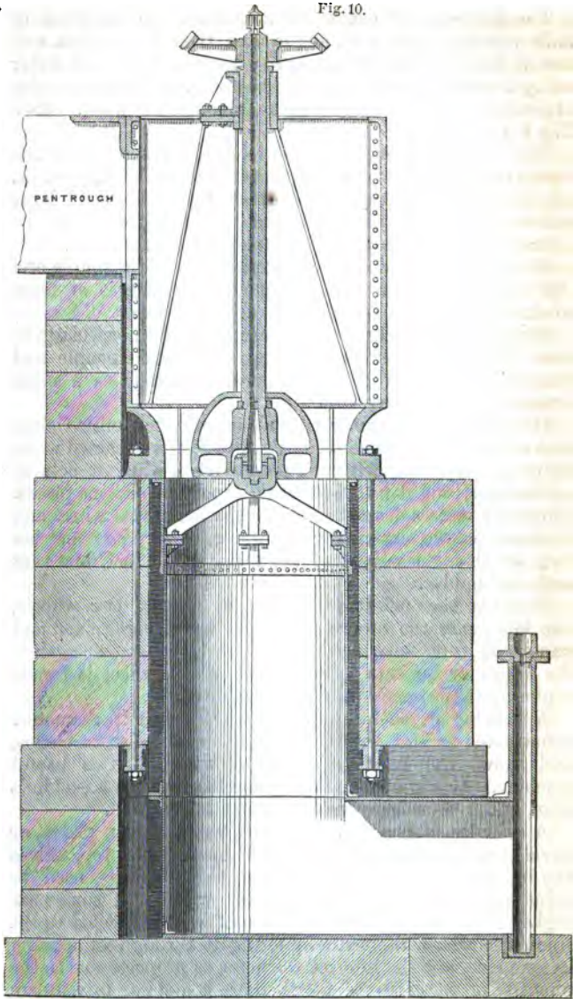
SECTIONAL ELEVATION.
